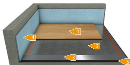
Underfloor heating (floating installation)
