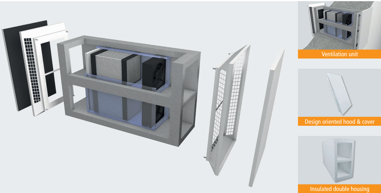
Insulated double housing
